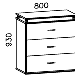
3 drawers w/file frame for A4 w/block & lock (without bottom) - max. weight per drawer: 35 kg
