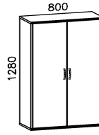
1 fixed shelf 1 adj. shelf
